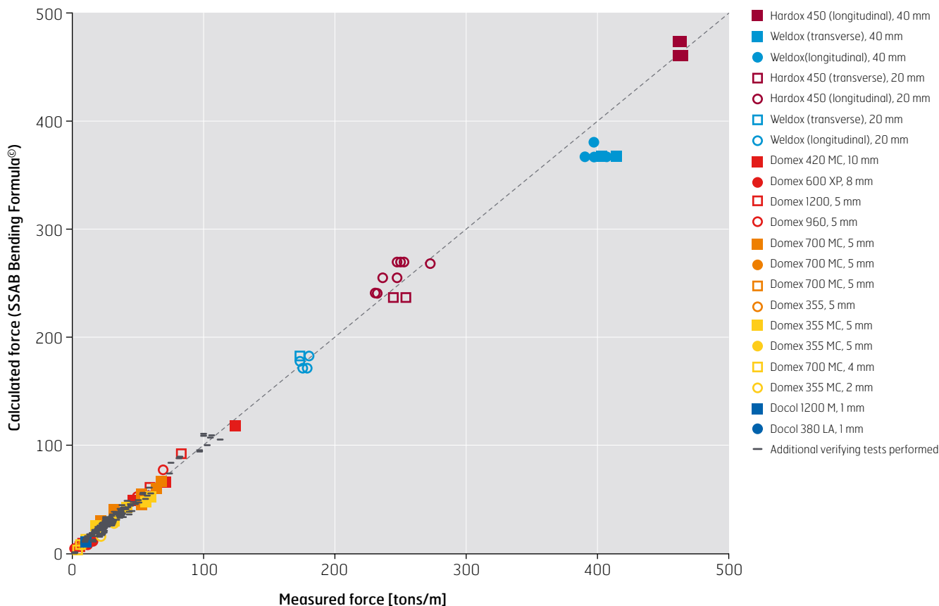
FIGURE 5 Bending force
